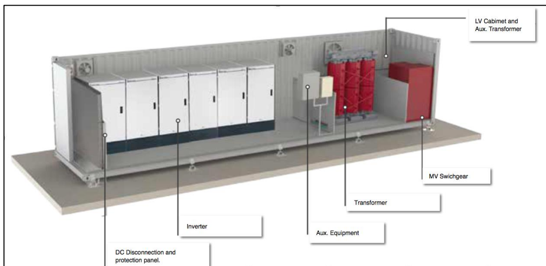
Photo 2-6: Option B – indoor equipment exterior (image reproduced courtesy of Power Electronics)
